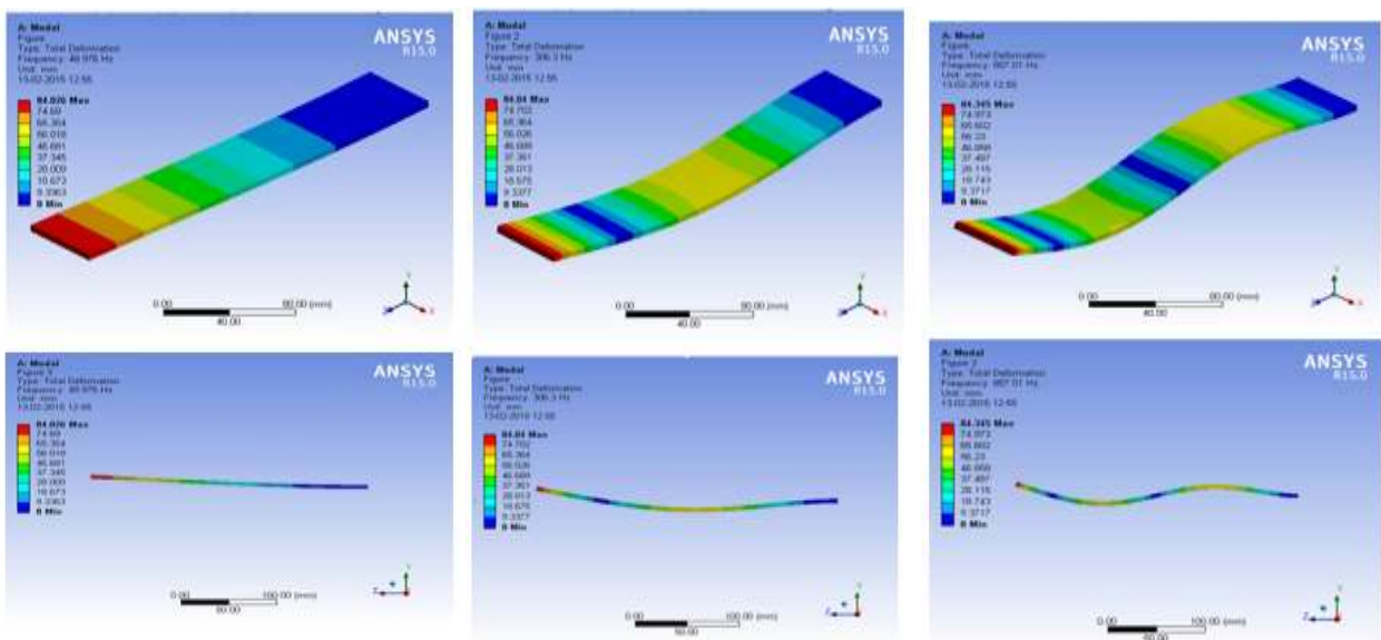
Fig. 3 (a): Mode 1 of cantilever beam (b) Mode 2 of cantilever beam (c) Mode 3 of cantilever beam
